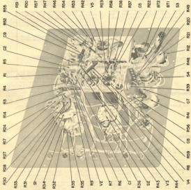
FIGURE 6.1 CHASSIS VIEW, MODEL 309A
