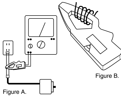
Figure 5-1. Amp-Clamp Connections
