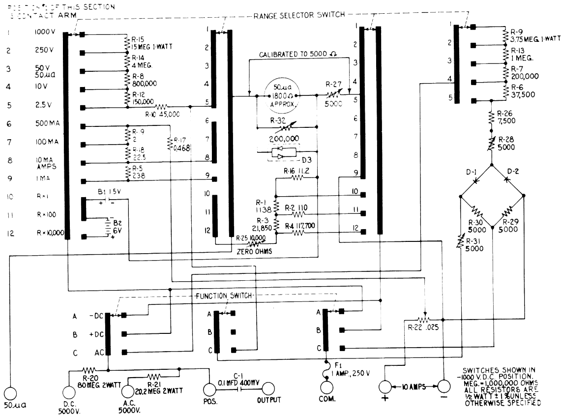
FIG. 8, OVERALL SCHEMATIC, SIMPSON VOLT-OHM-MILLIAMMETER, 260 SERIES 5 & SERIES 5M
