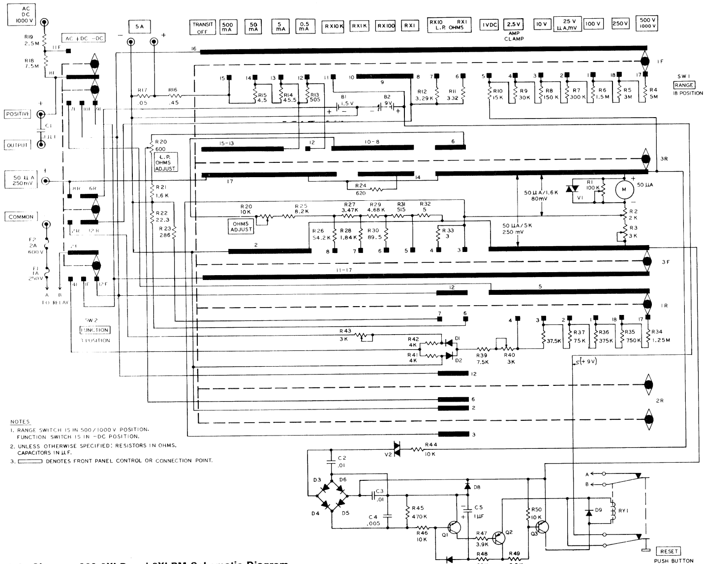
Figure 6-1. Simpson 260-6XLP and 6XLP Schematic Diagram
