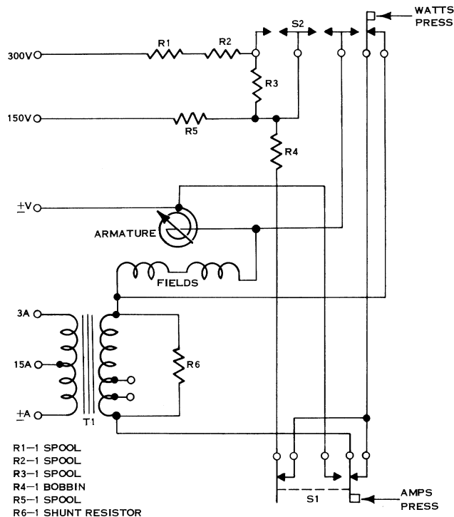
Figure 7-1. Model 390-2, Schematic Diagram
