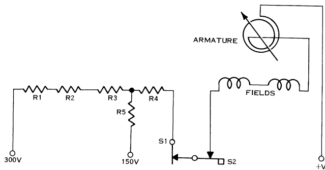
Figure 5-1. Simplified Voltmeter Circuit
