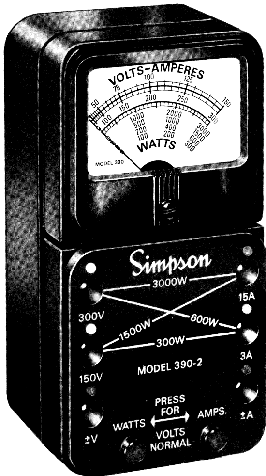
Figure 1-1. Model 390-2 Volt-Amp-Wattmeter
