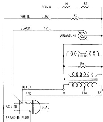
Figure 5-3. Simplified Wattmeter Circuit, 300 Watt Range
